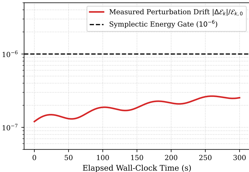
(b) Mukhanov-Sasaki Energy Balance ( \leq 10^{-6} )
