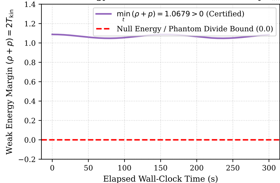
(c) Weak Energy Condition via Metric Positivity \tau_{im} > 0
